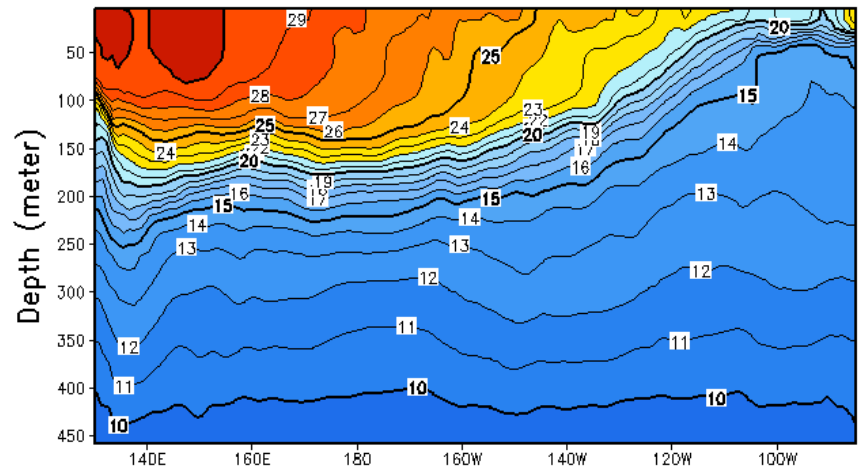
Equatorial Temperature (°C), Nov 24 2016
