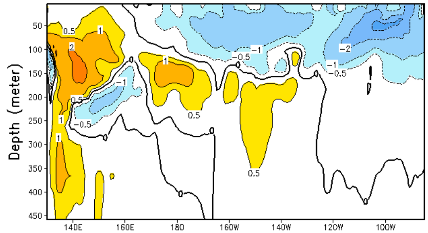
Equatorial Temperature Anom (°C), Nov 24 2016
